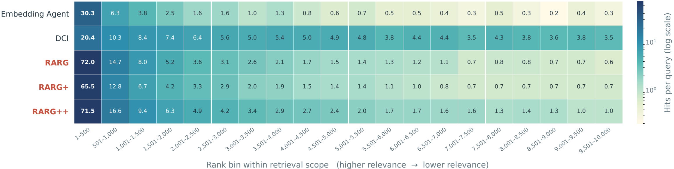
BrowseComp-Plus (100K): Scope-Hit Distribution by Rank
