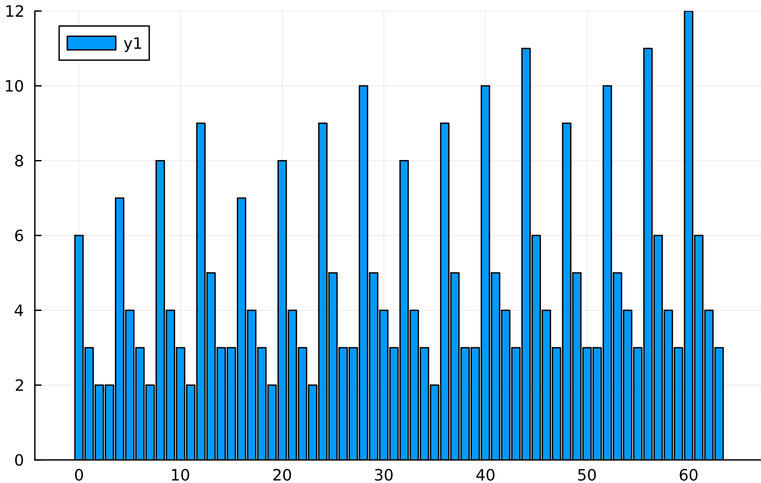
Dirichlet plot
