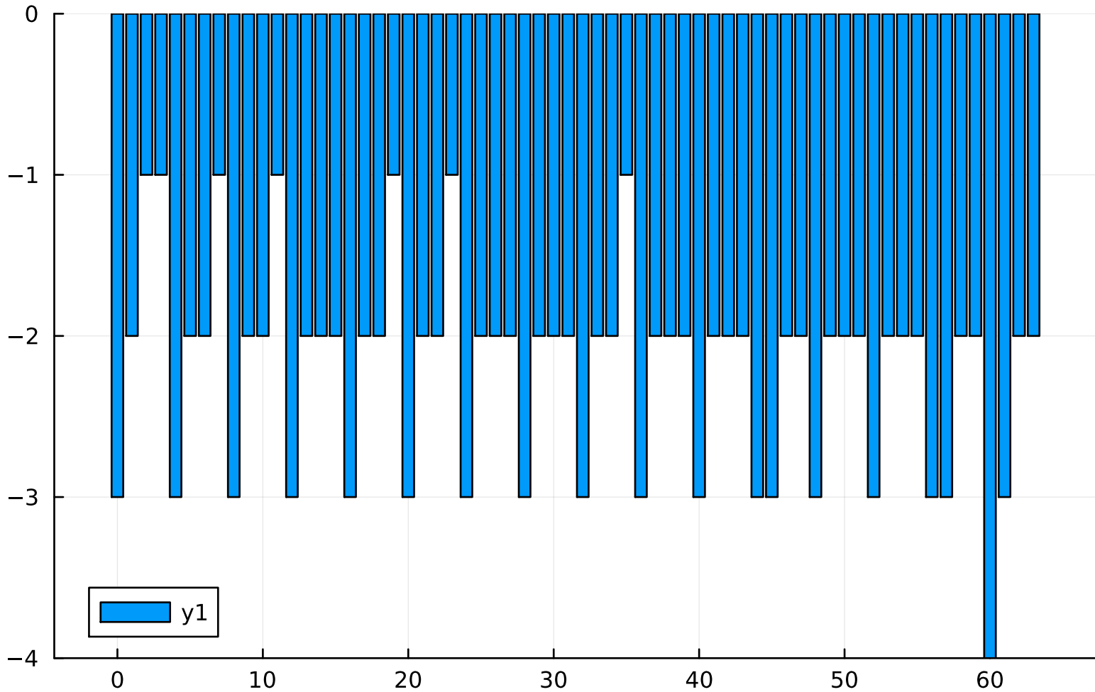
Dirichlet plot
