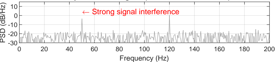
Analysis 2: Welch Method (Hamming window, L=256)
