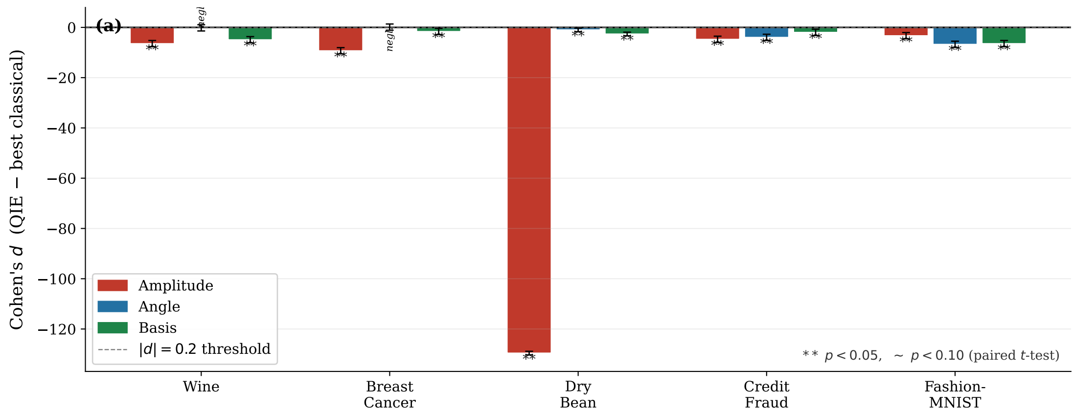
Effect sizes: QIE vs. best classical baseline per dataset
