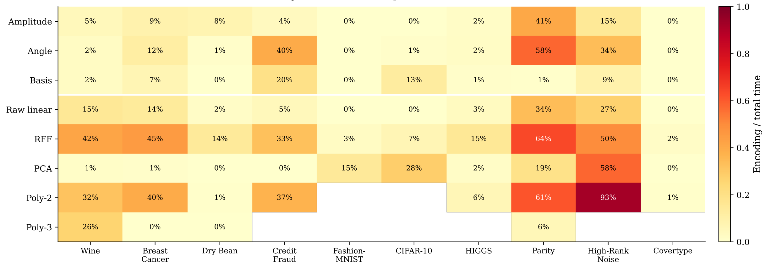
Encoding overhead fraction per method and dataset
