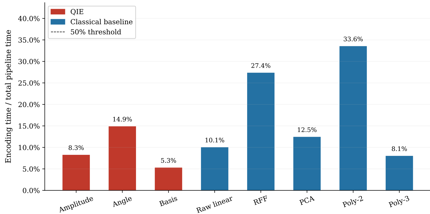
Encoding overhead fraction (mean across datasets)
