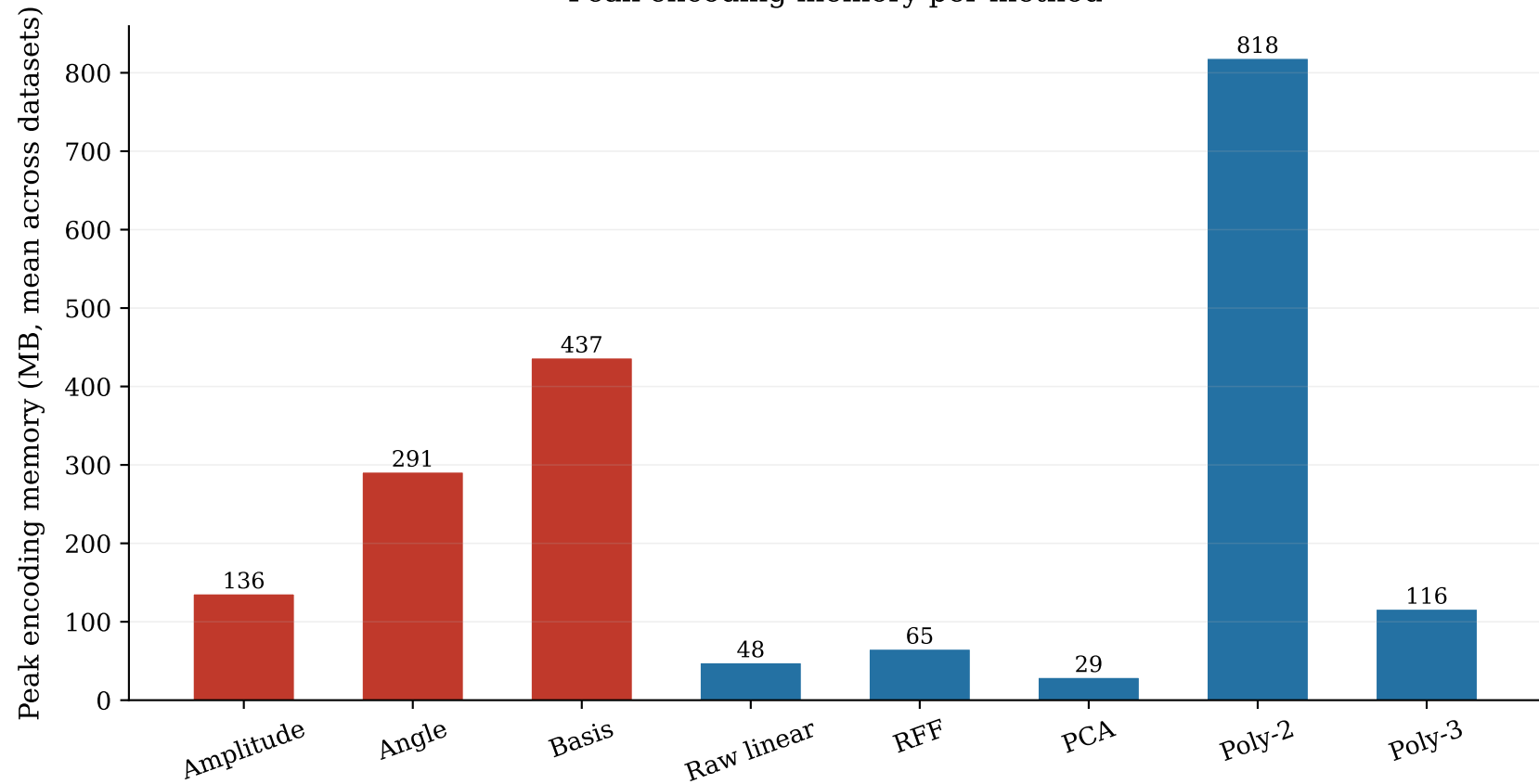
Peak encoding memory per method
