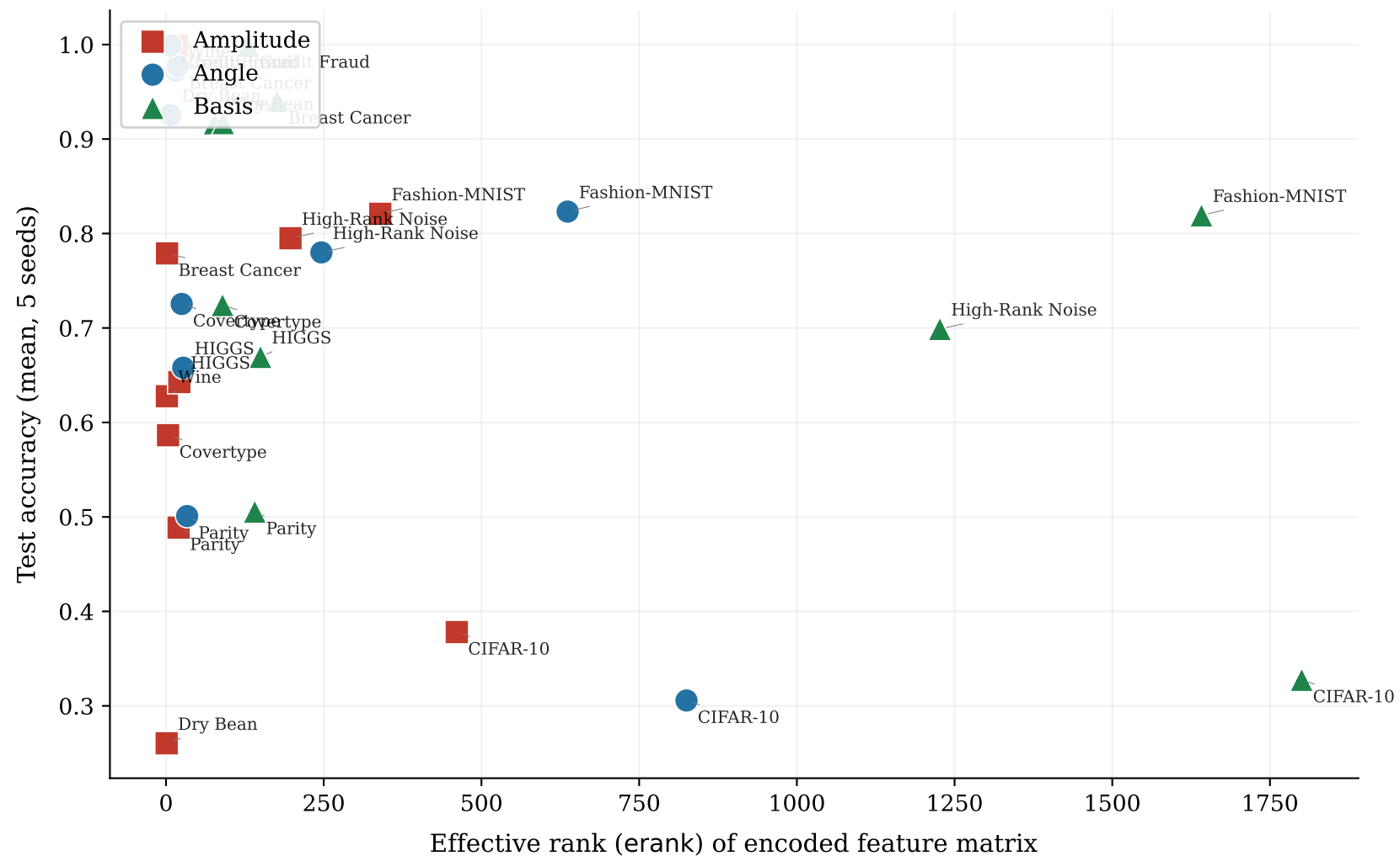
Feature-space effective rank vs. classification accuracy
