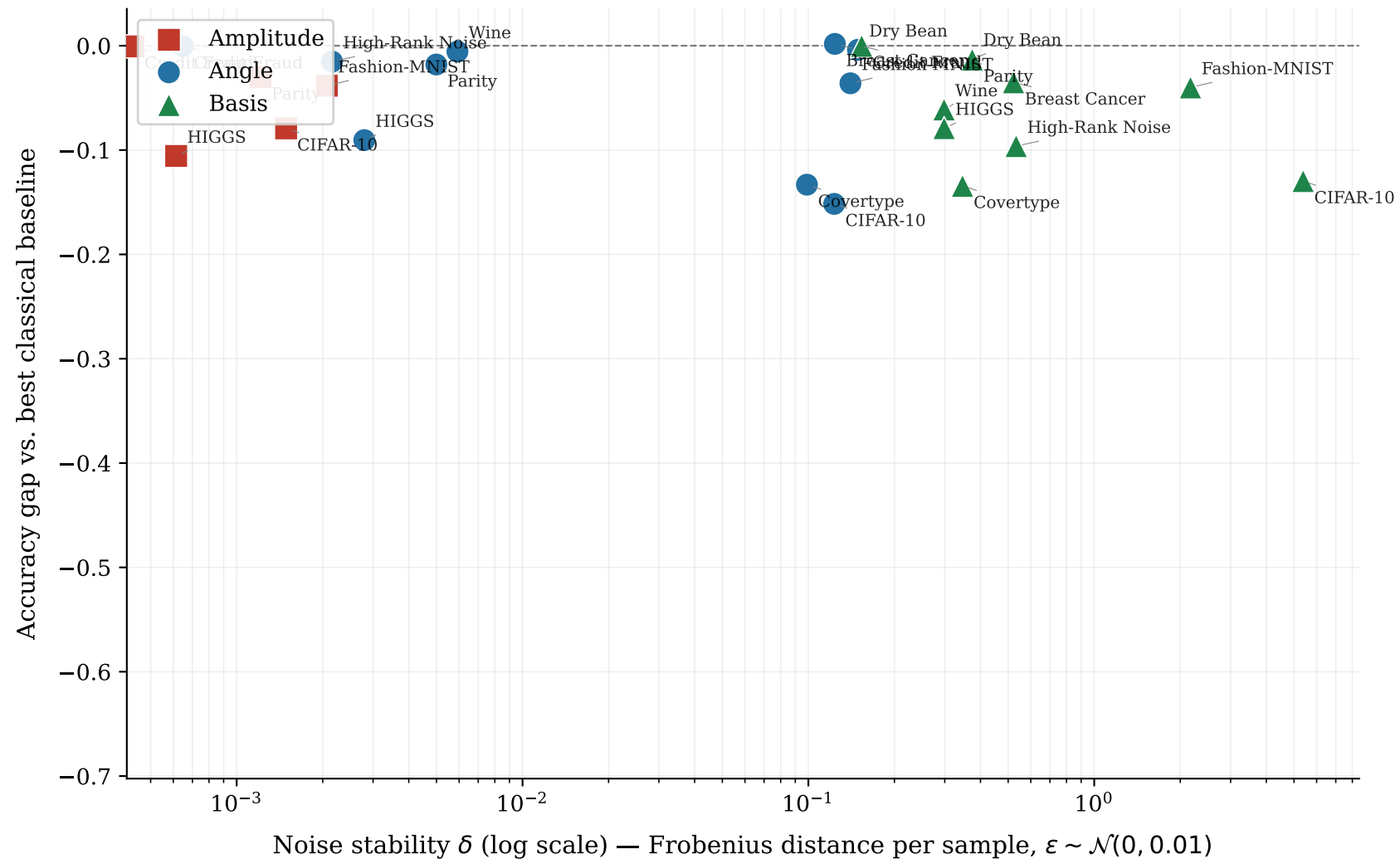
Noise sensitivity vs. QIE accuracy gap
