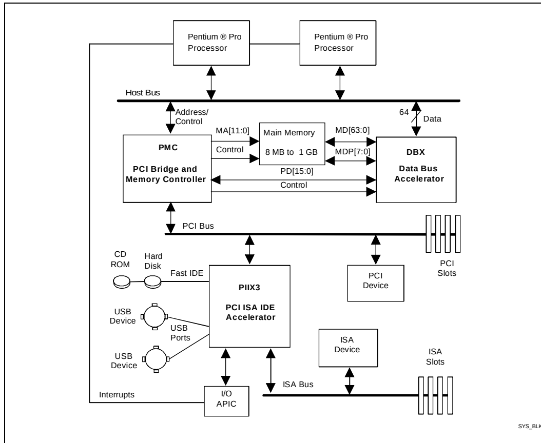
Figure 1. 440FX PCIsset System Block Diagram
