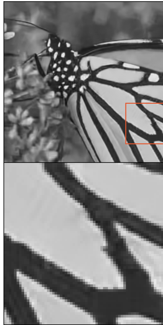
BM3D 29.40 dB
