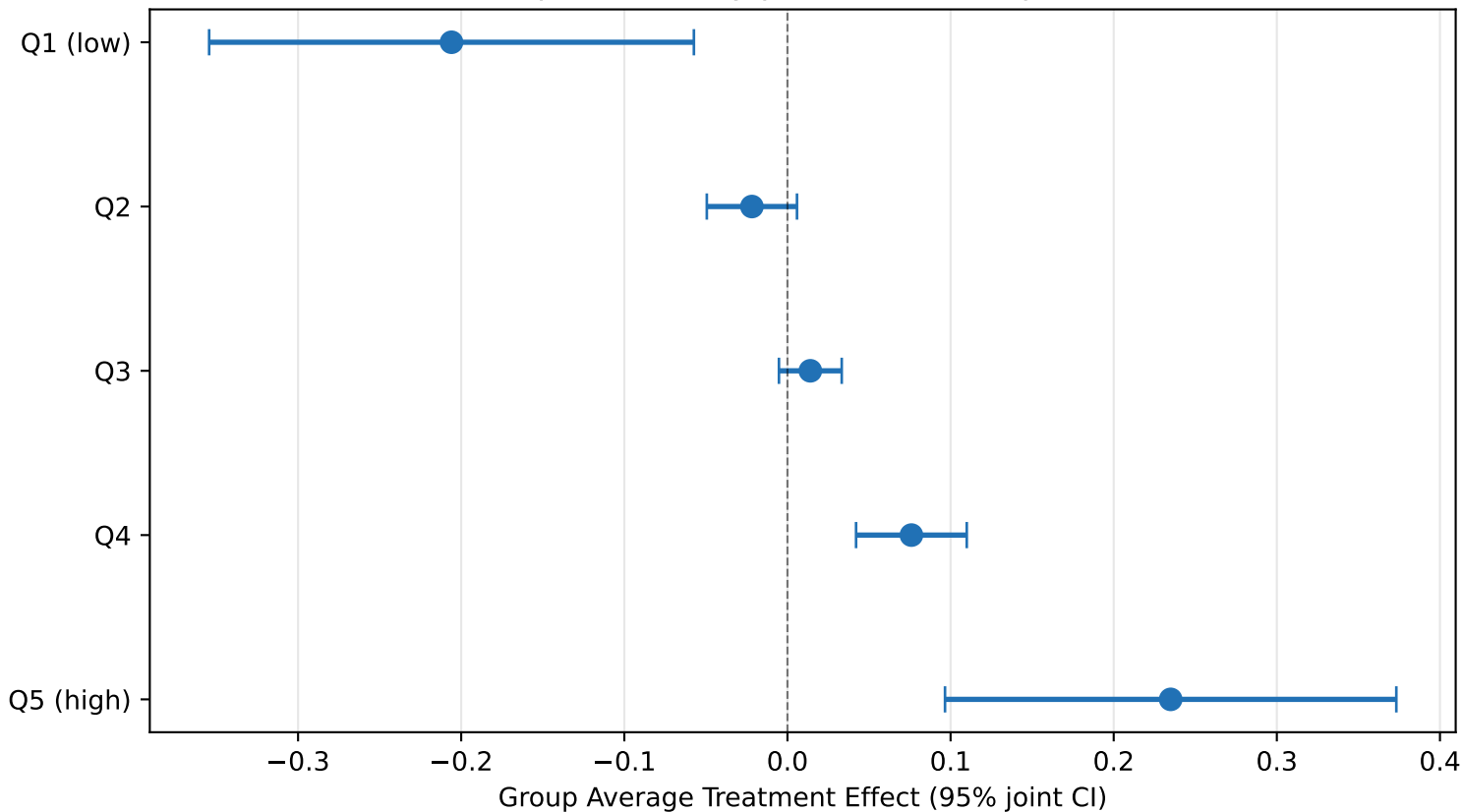
GATE: skill1_corr \hat{\tau} ' growth Groups defined by predicted CATE quintiles
