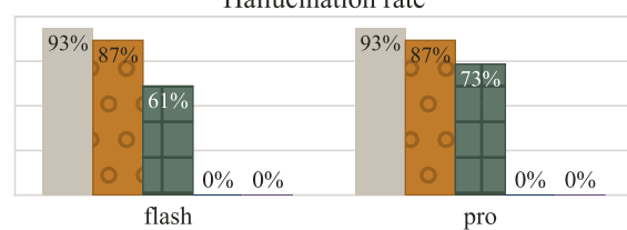
Hallucination rate
