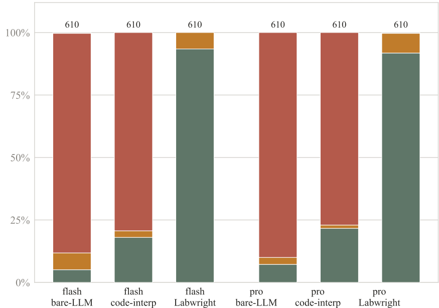
Outcome classes (confusion matrix → CER)
