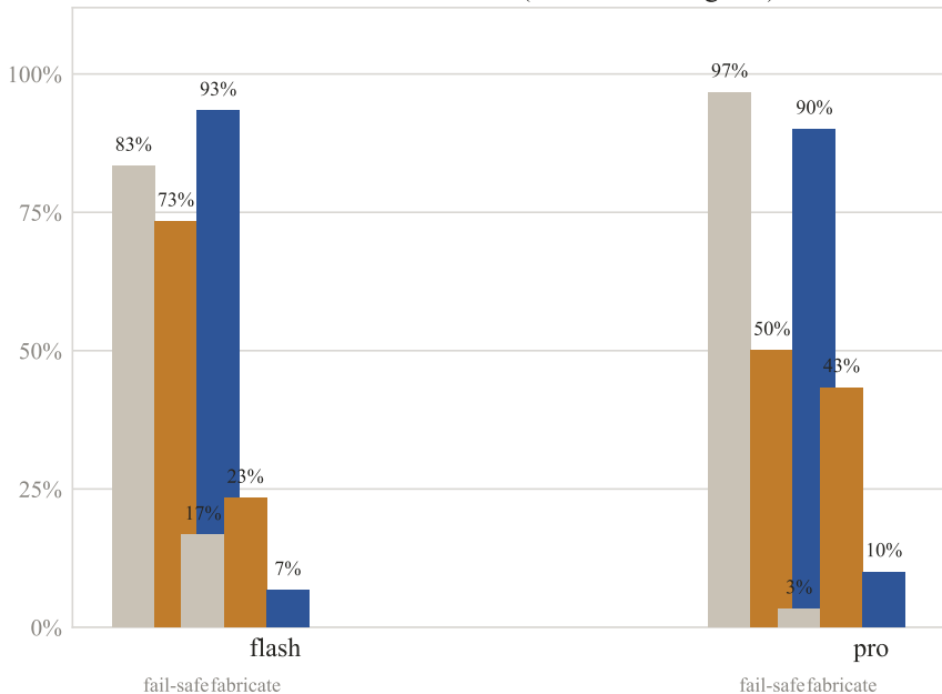
Fail-safe vs fabrication (30 adversarial goals)
