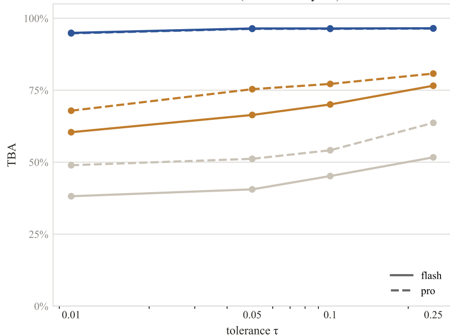
TBA- \tau curve (full 610-entry set)
