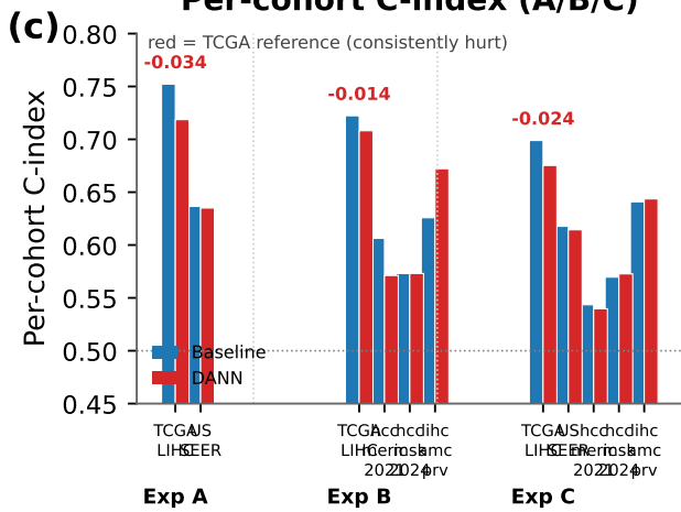
Per-cohort C-index (A/B/C)
