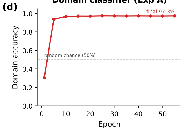
Domain classifier (Exp A)
