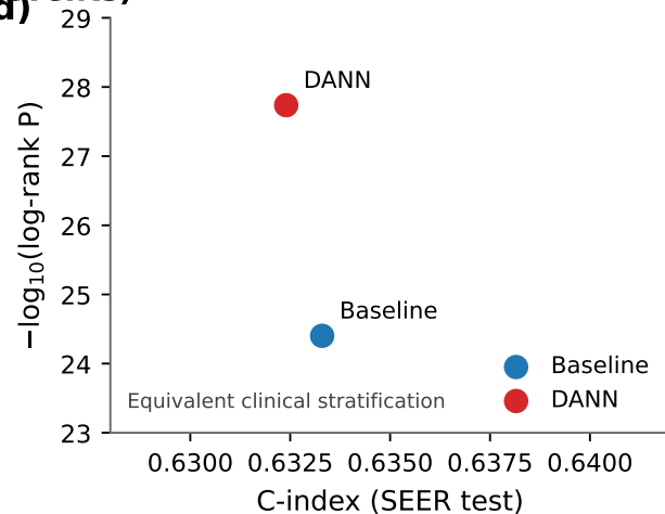
Stratification statistics (SEER test, n=1,500, 1,162 events)
