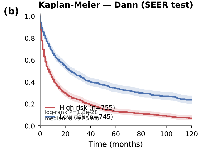
Stratification statistics (SEER test, n=1,500, 1,162 events)
