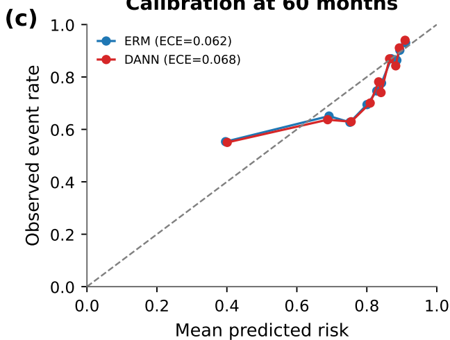
Calibration at 60 months
