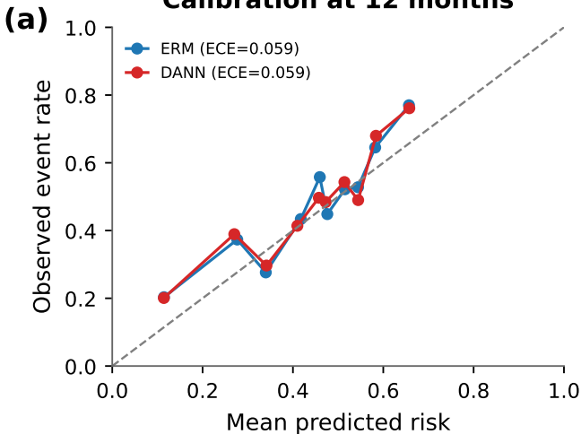
Calibration at 12 months
