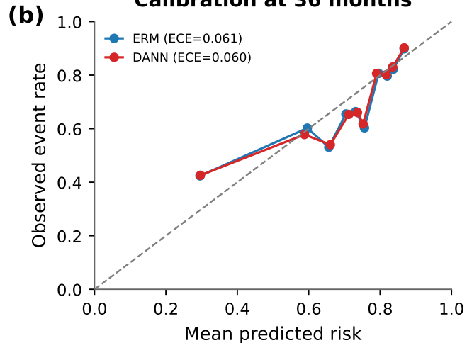
Calibration at 36 months
