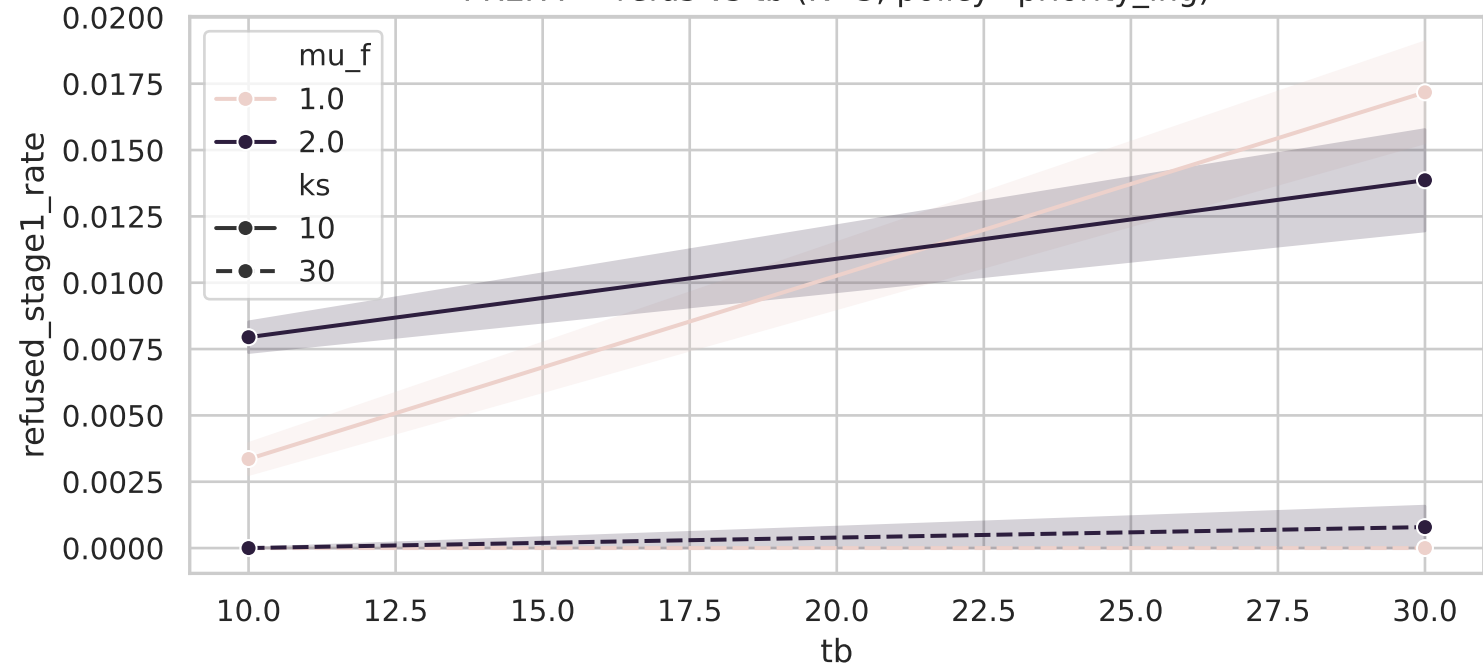
PREPA — refus vs tb (K=3, policy=priority_ing)
