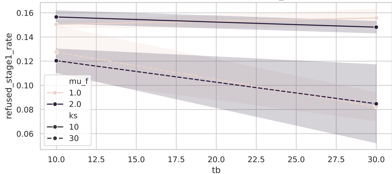
PREPA — refus vs tb (K=4, policy=split_servers)
