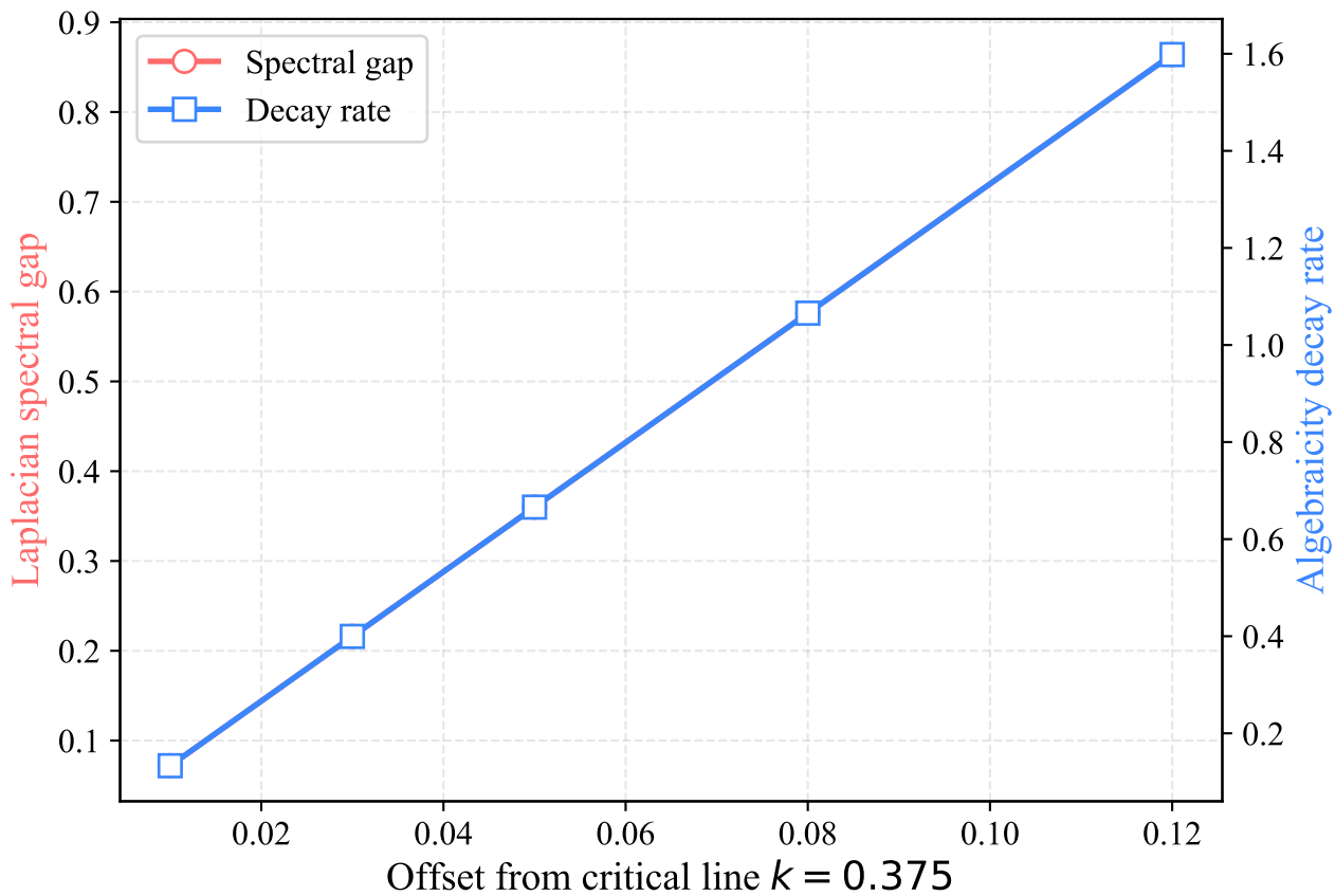
Spectral Gap vs Algebraicity Decay Rate (Weil-Petersson Metric)
