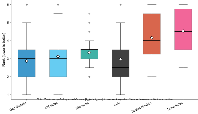
Figure 2. Rank Distribution Across Datasets
