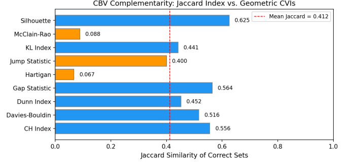
Fig. 4. Jaccard similarity between CBV and each geometric CVI, indicating substantial independence.
