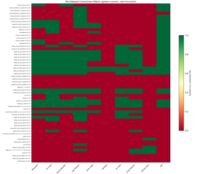
Fig. 5. Correctness heatmap across all indices and datasets. Green (correct) and red (incorrect) reveal divergent success regimes.
