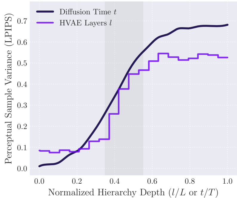
CIFAR-10
