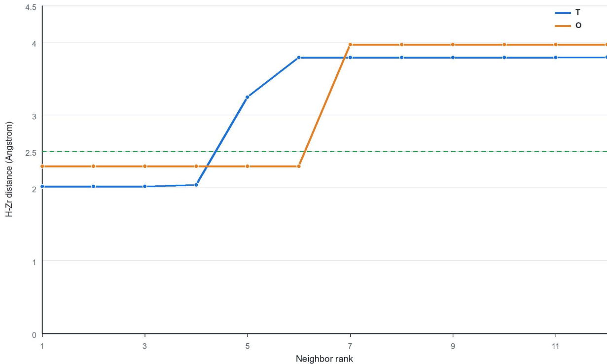
Sorted H-Zr neighbor distances
