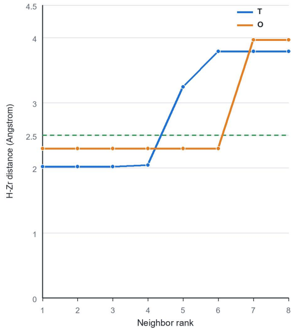
Local coordination
