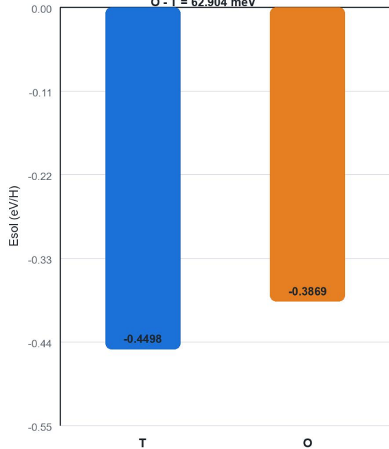
Site energetics
