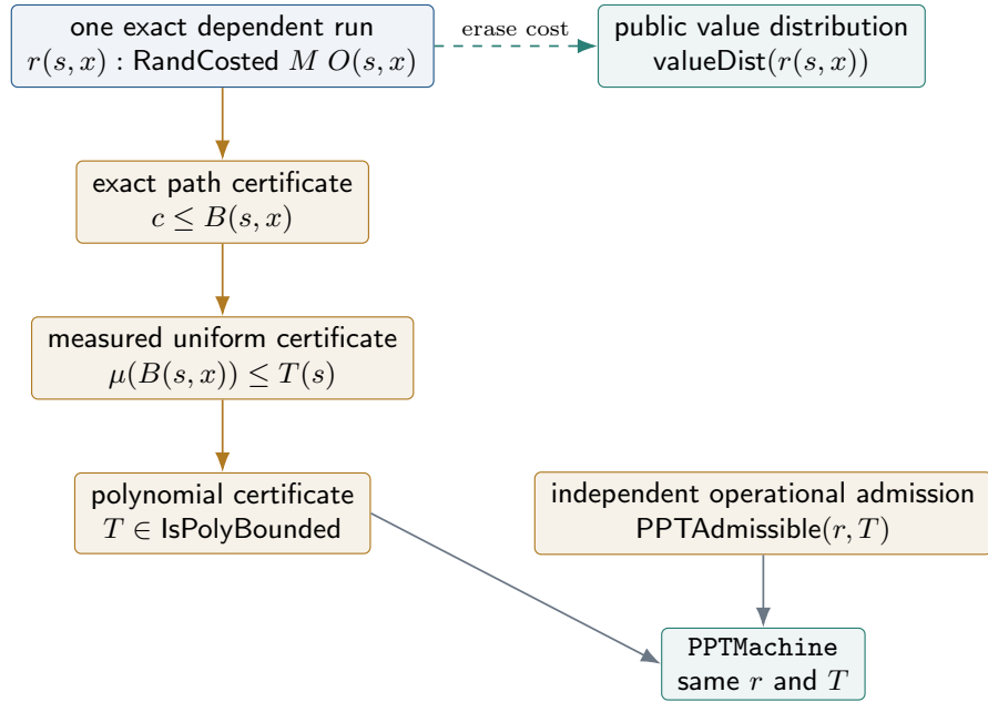
Fig. 3. Certificate refinement never rewrites the exact run. Polynomial annotation and independent operational admission must both be present at the PPT boundary; probability erasure is orthogonal.
