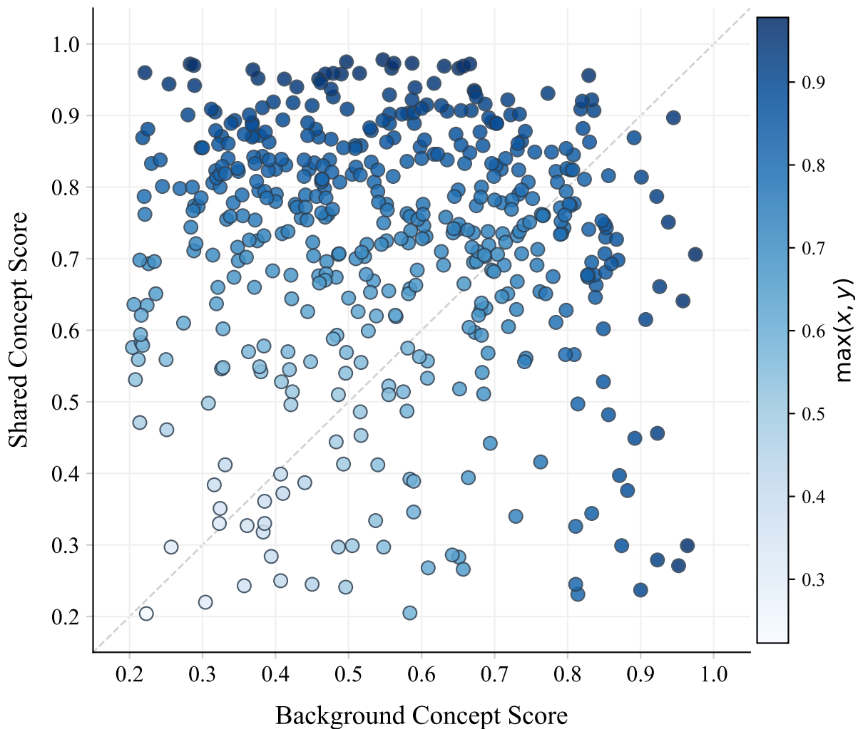
Distribution Analysis of Concept Score
