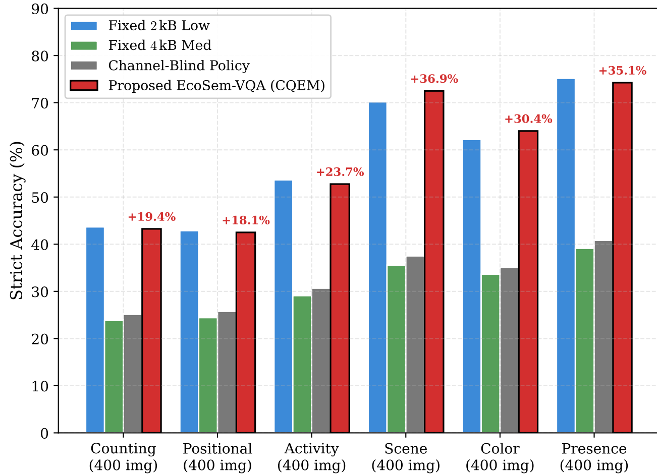
(a) Channel Outage Robustness by Task ( \gamma = 5.0 dB, CQEM)
