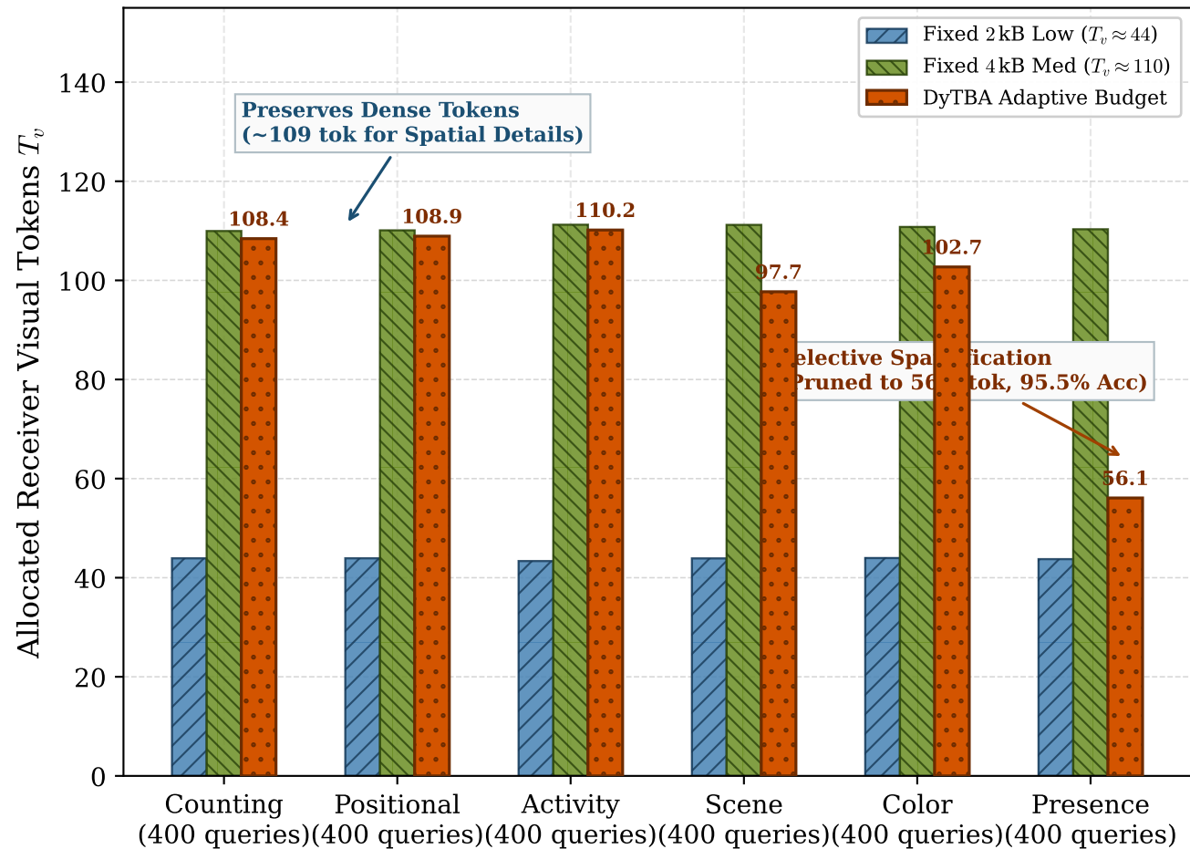
(b) DyTBA Visual Token Budget Allocation ( T_v ) by Semantic Demand
