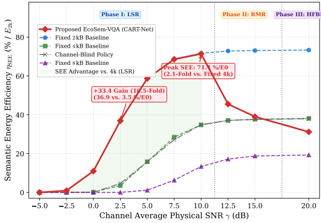
Fig. 4. Semantic Energy Efficiency ( \eta_{SEE} , % accuracy per unit energy) versus channel SNR \gamma . CART-Net delivers up to a 10.5-fold energy efficiency advantage (+33.4 margin) over fixed 4k under severe fading ( \gamma = 2.5 dB) via PPC power concentration.
