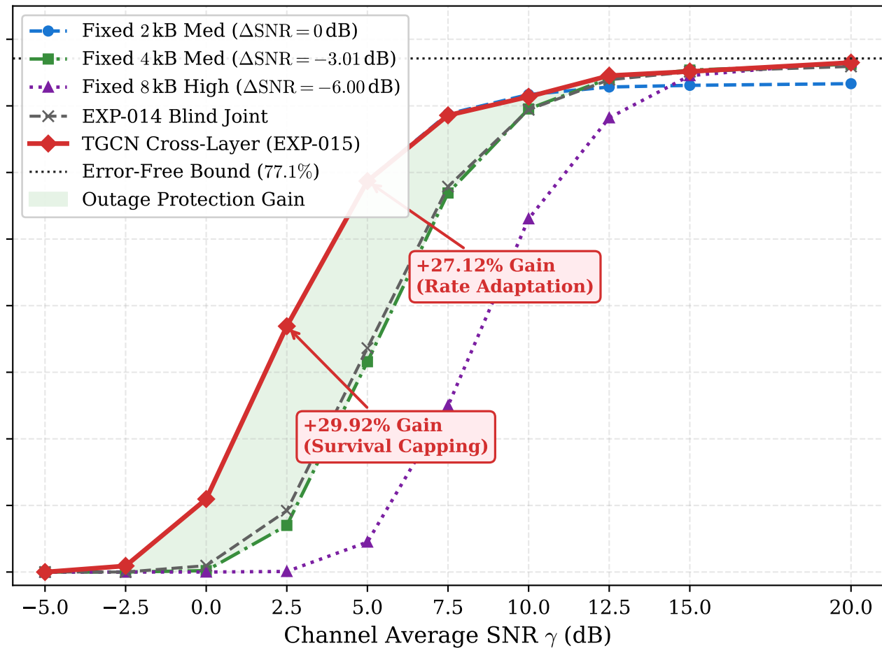
(b) Mode 2: Constant Transmission Energy Budget ( E_{tx} = E_0 )
