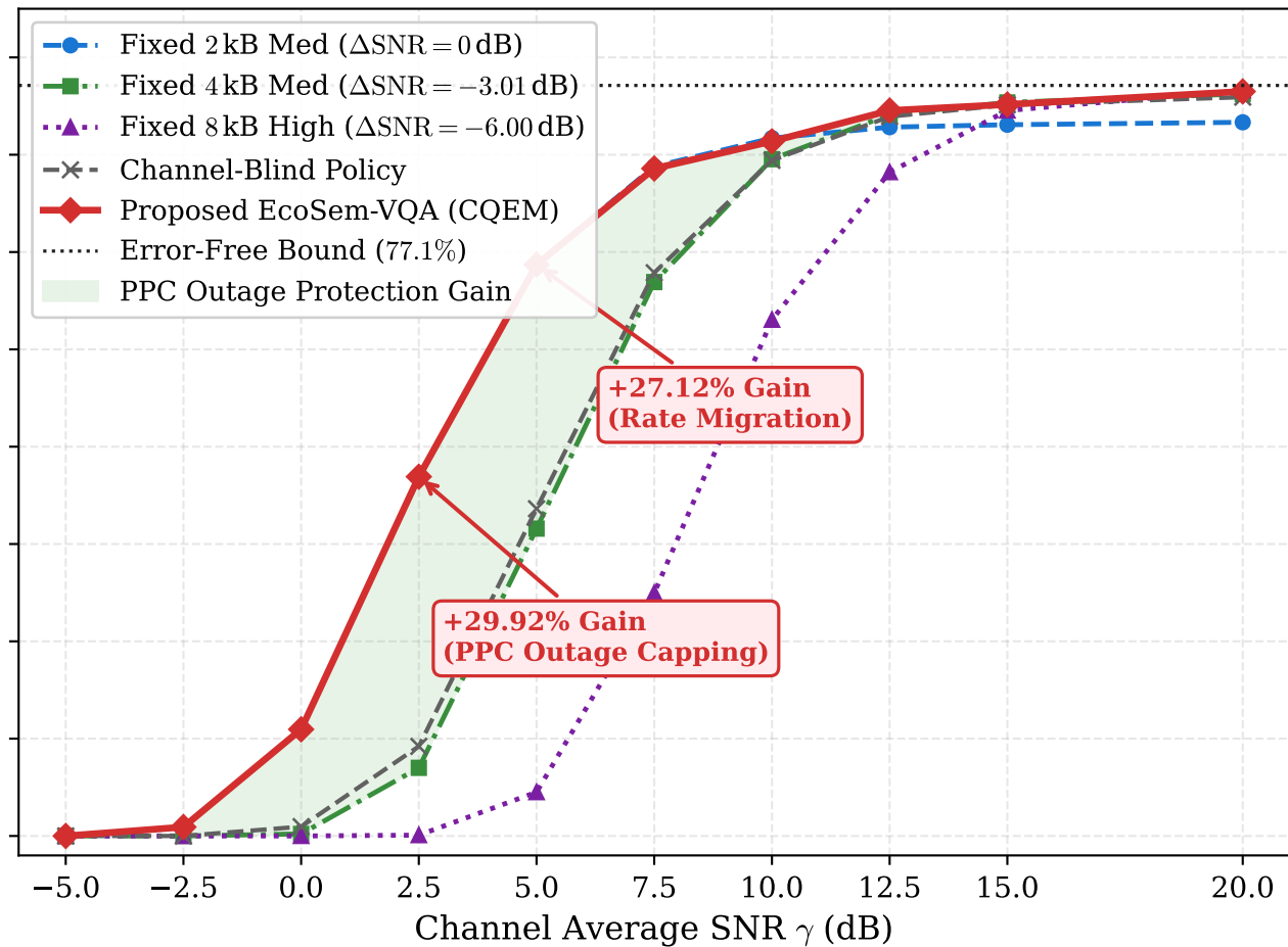
(b) CQEM: Constant Query-Energy Budget ( E_{tx} = E_0 )
