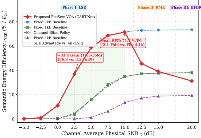
Fig. 4. Semantic Energy Efficiency ( \eta_{SEE} , % accuracy per unit energy) versus channel SNR \gamma . CART-Net delivers up to a 10.5-fold energy efficiency advantage (+33.4 margin) over fixed 4k under severe fading ( \gamma = 2.5 dB) via PPC power concentration.
