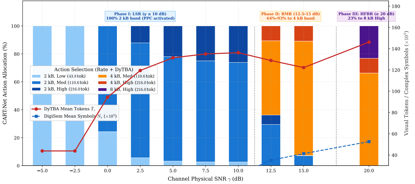
Fig. 1. Empirical dynamic action routing distribution and emergent three-phase adaptation mechanics of EcoSem-VQA across 2,400 blind test images over Rician fading ( K = 6 dB): Link Survival Regime (LSR, \leq 10 dB), Rate Migration Regime (RMR, 12.5 \sim 15 dB), and High-Fidelity Burst Regime (HFBR, \geq 20 dB). The overlaid curves show the mean DyTBA receiver visual token budget T_v and mean complex channel symbols N_s .
