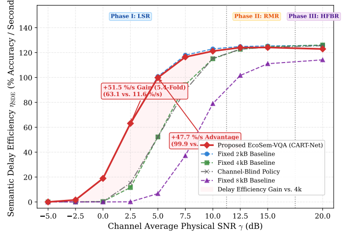
Fig. 5. Semantic Delay Efficiency ( \eta_{SDE} , % accuracy per second) versus channel SNR \gamma , demonstrating superior end-to-end task throughput enabled by DyTBA visual token pruning and adaptive channel coding.
