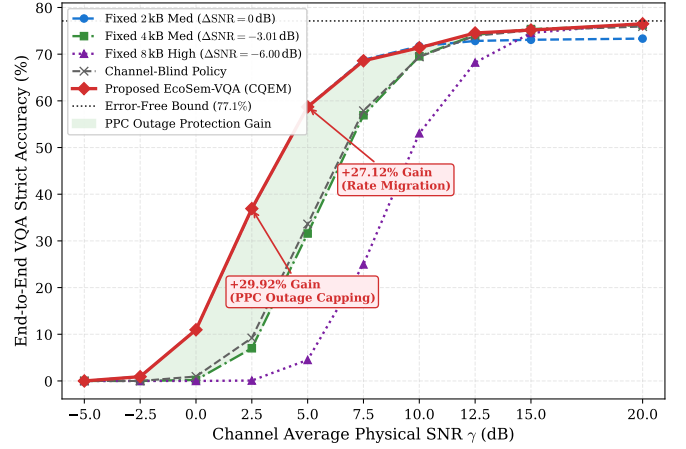
Fig. 3. End-to-End VQA Strict Accuracy (%) versus channel SNR \gamma (dB) under Constant Query-Energy Mode (CQEM, E_{tx} = E_0 ). Physical Power Concentration (PPC) concentrates RF power on compact payloads, delivering up to +29.92% and +27.12% accuracy gains over static 4k under fading.
