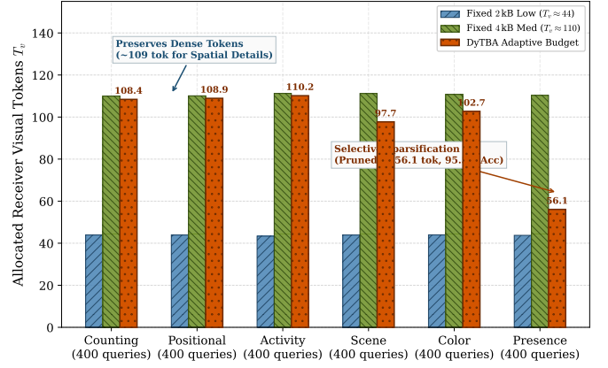
Fig. 7. Receiver visual token budget T_v allocated by DyTBA across question categories. DyTBA autonomously discovers task visual entropy, pruning presence queries to 56.1 tokens while preserving dense spatial tokens (~109 tokens) for counting and positional reasoning.
