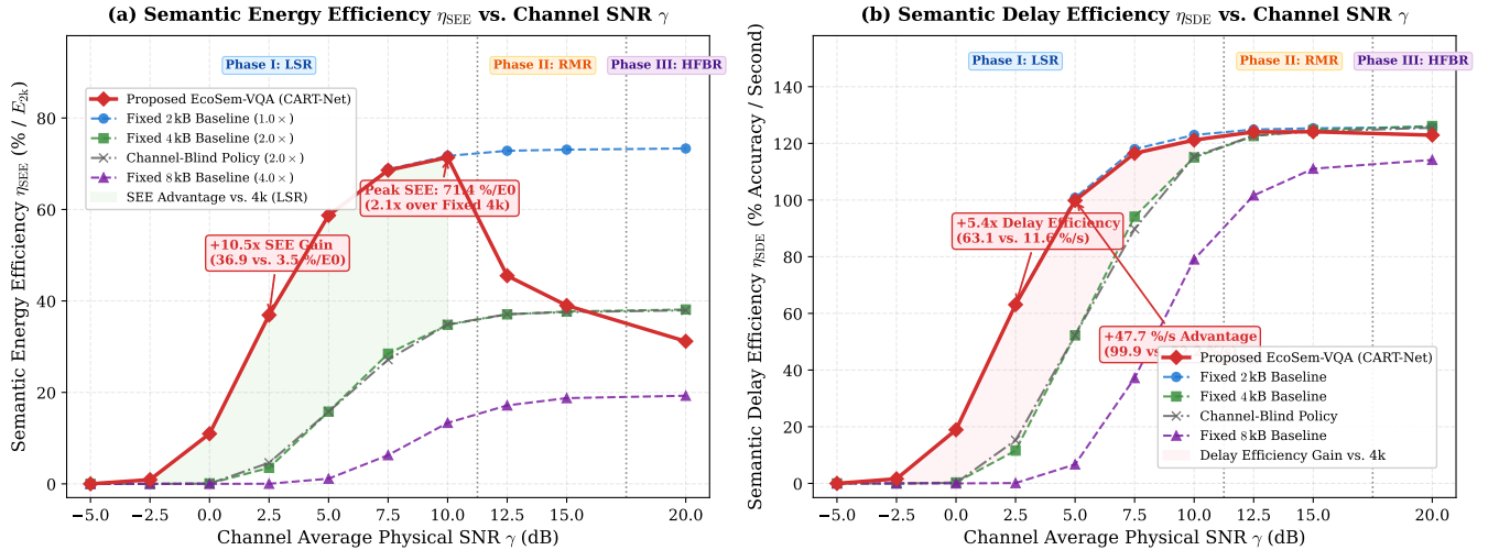
Fig. 3. Semantic energy and delay efficiency metrics across the channel physical SNR continuum from \gamma = -5.0 dB to 20.0 dB. (a) Semantic Energy Efficiency ( \eta_{SEE} = \text{Accuracy}/(E_{tx}/E_{2k}) , % per unit energy) versus channel SNR \gamma . CART-Net delivers up to a 10.5 \times energy efficiency advantage over fixed 4k under severe fading ( \gamma = 2.5 dB) via PPC power concentration and reaches peak efficiency (71.4) at 10 dB. (b) Semantic Delay Efficiency ( \eta_{SDE} = \text{Accuracy}/t_{e2e} , % accuracy per second) versus channel SNR \gamma , demonstrating superior end-to-end task throughput enabled by DyTBA visual token pruning and adaptive channel coding.
