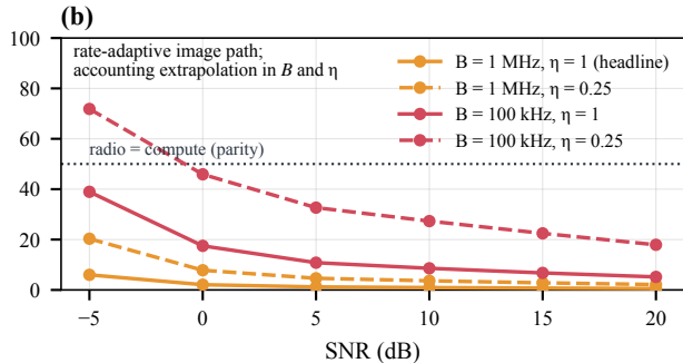
radio share of per-answer energy (%)
