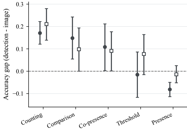
● VisDrone: three channels □ DroneVehicle: Rician (b) Paired gap and 95% cluster CI
