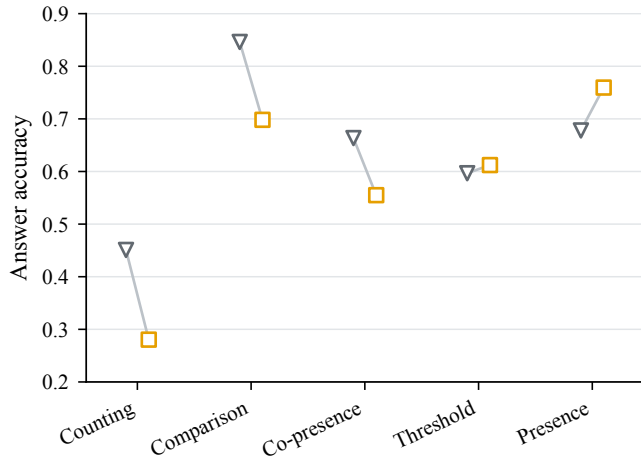
▽ Fixed detection evidence □ Rate-adaptive image (a) Branch accuracy on VisDrone
