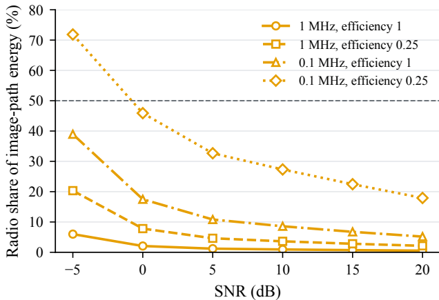
(a) Bandwidth and amplifier efficiency
