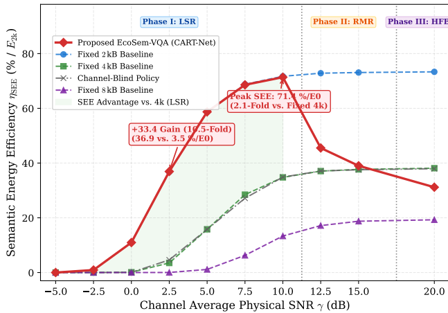
Fig. 3. Semantic Energy Efficiency ( \eta_{SEE} , % accuracy per unit energy) versus channel SNR \gamma . CART-Net delivers up to a 10.5-fold energy efficiency advantage (+33.4 margin) over fixed 4k under severe fading ( \gamma = 2.5 dB) via PPC power concentration.
