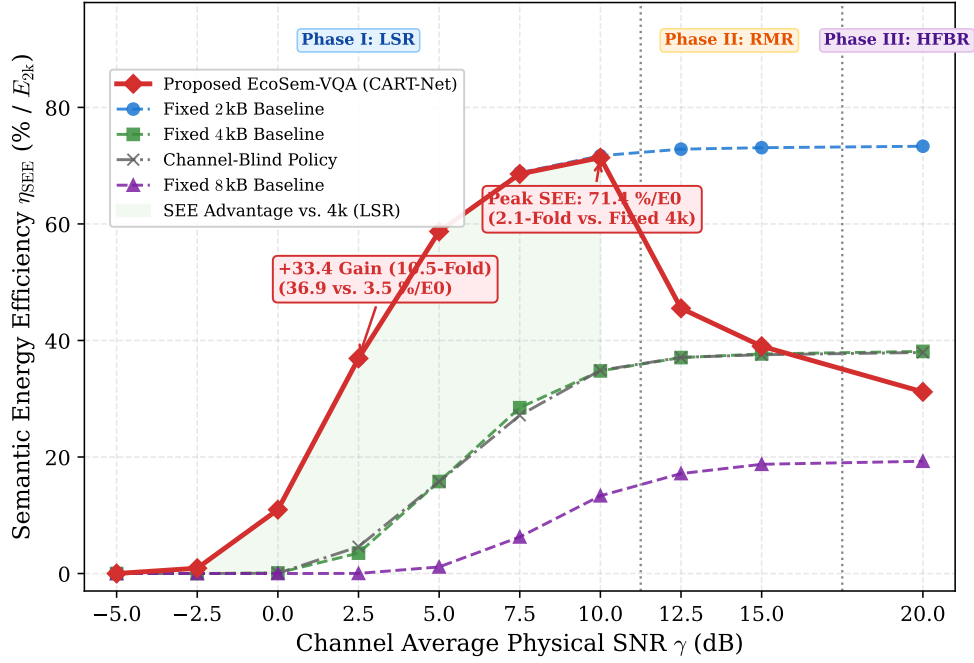
Fig. 3. Semantic Energy Efficiency ( \eta_{SEE} , % accuracy per unit energy) versus channel SNR \gamma . CART-Net delivers up to a 10.5-fold energy efficiency advantage (+33.4 margin) over fixed 4k under severe fading ( \gamma = 2.5 dB) via PPC power concentration.
