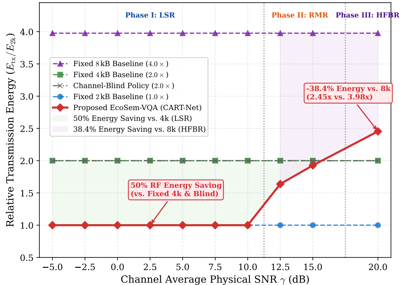
(a) Relative RF Transmission Energy ( E_{\text{tx}}/E_{2k} ) vs. Channel SNR \gamma
