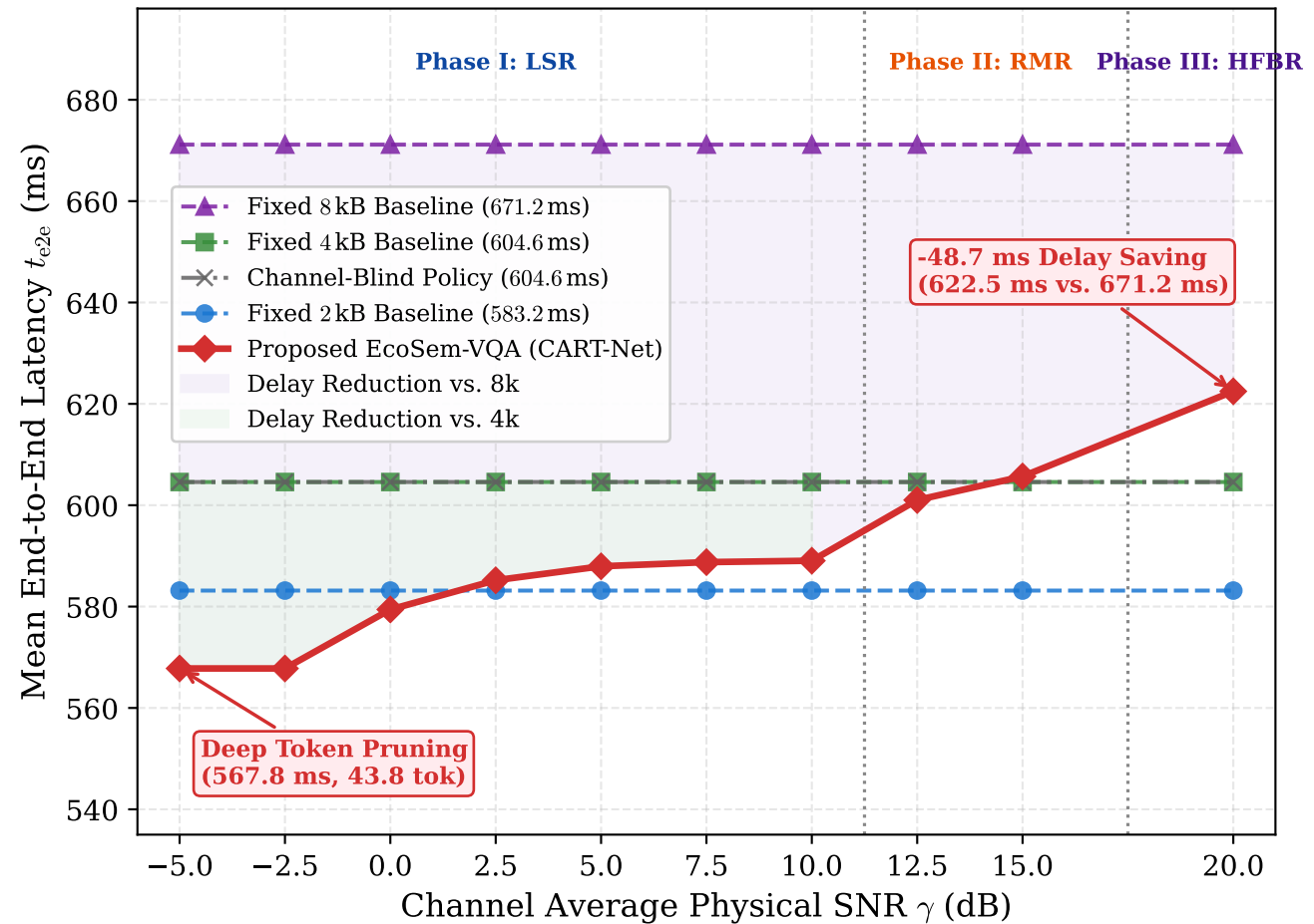
(b) Mean End-to-End Latency t_{e2e} (ms) vs. Channel SNR \gamma
