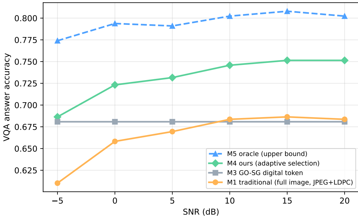
Accuracy vs SNR (Rician K=6 dB)
