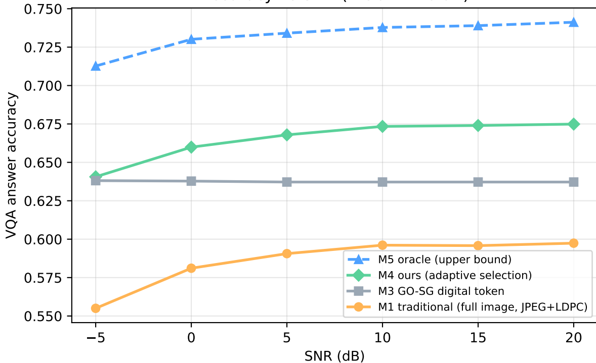
Accuracy vs SNR (Rician K=6 dB)
