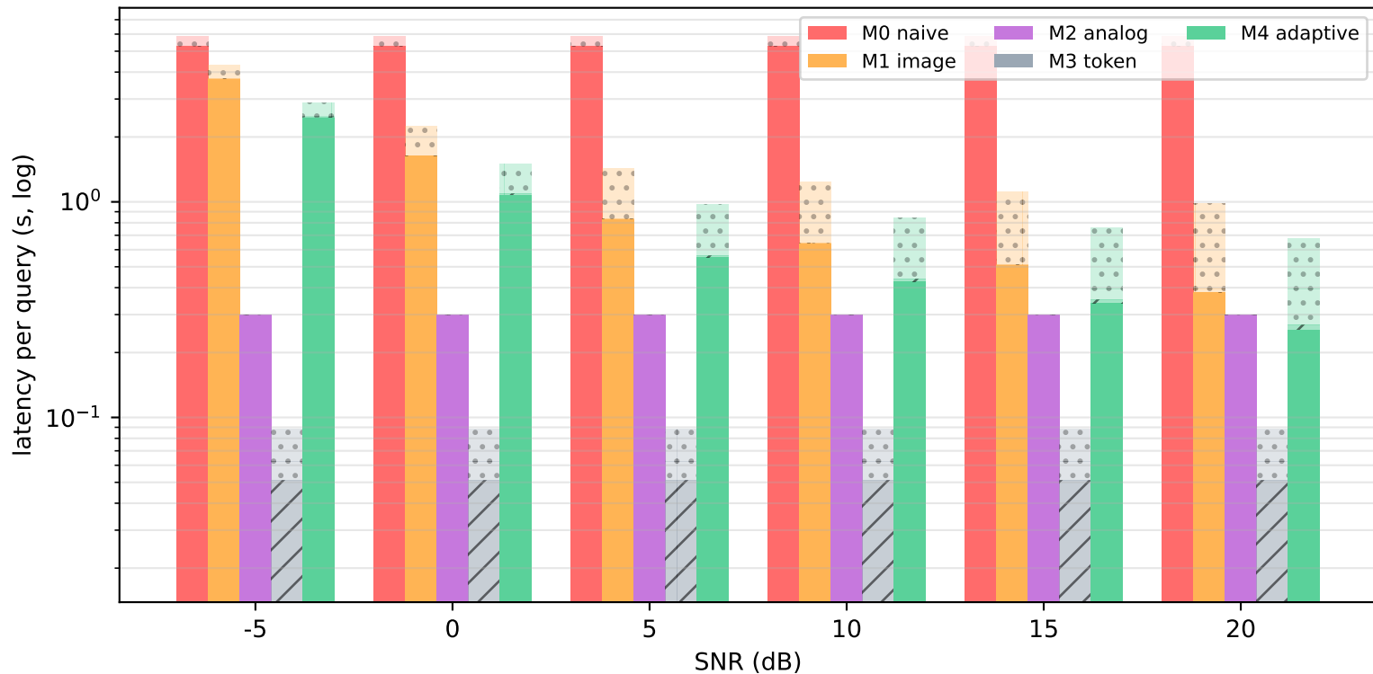
End-to-end latency breakdown (rayleigh); solid=upload, //=tx-side detector, ..=inference
