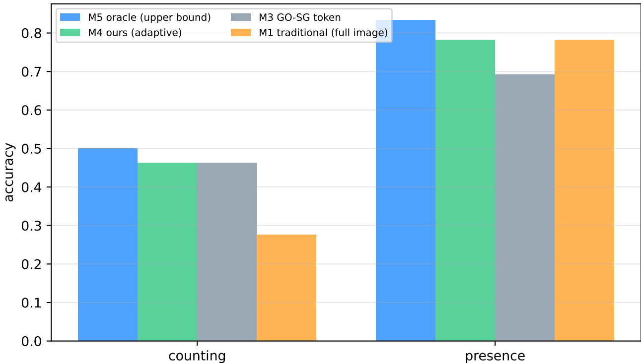
Per-question-type accuracy (Rician K=6 dB, SNR=5 dB)
