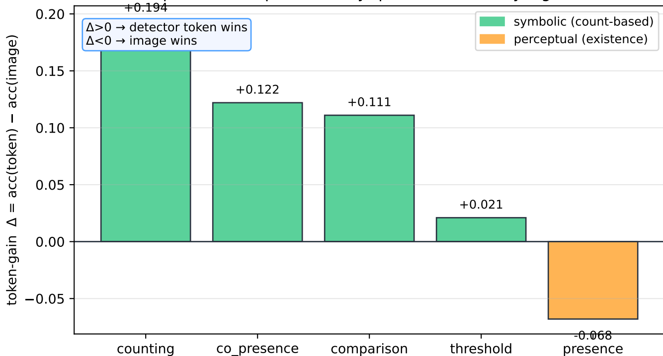
Evidence-question complementarity (pooled AWGN/Rayleigh/Rician, test)
