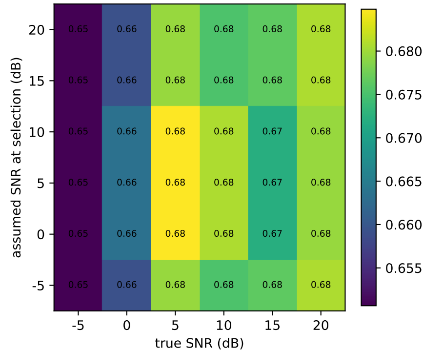
Rician K=6 dB
