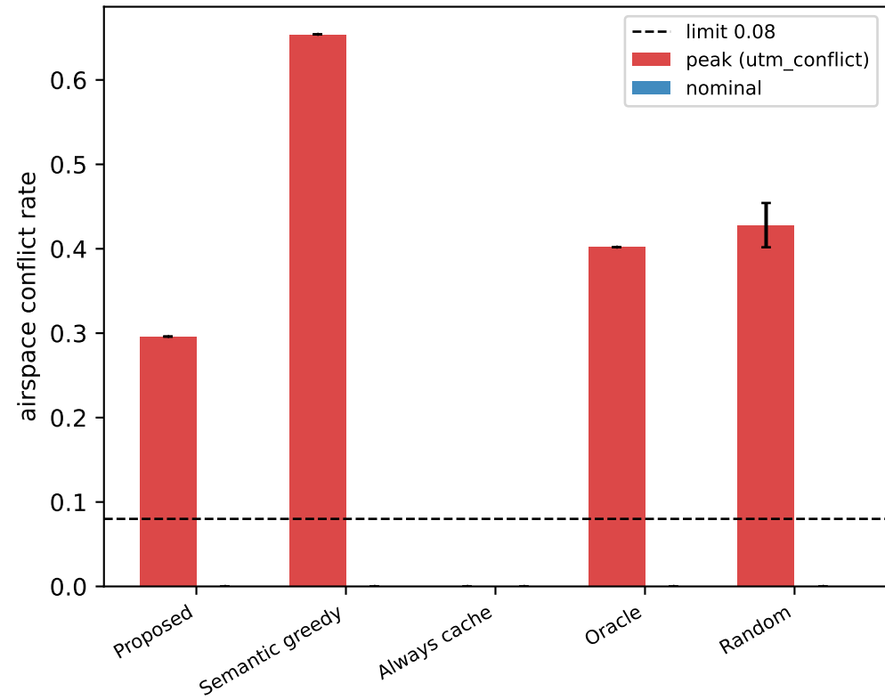
(a) Constraint violation, dual conditions
