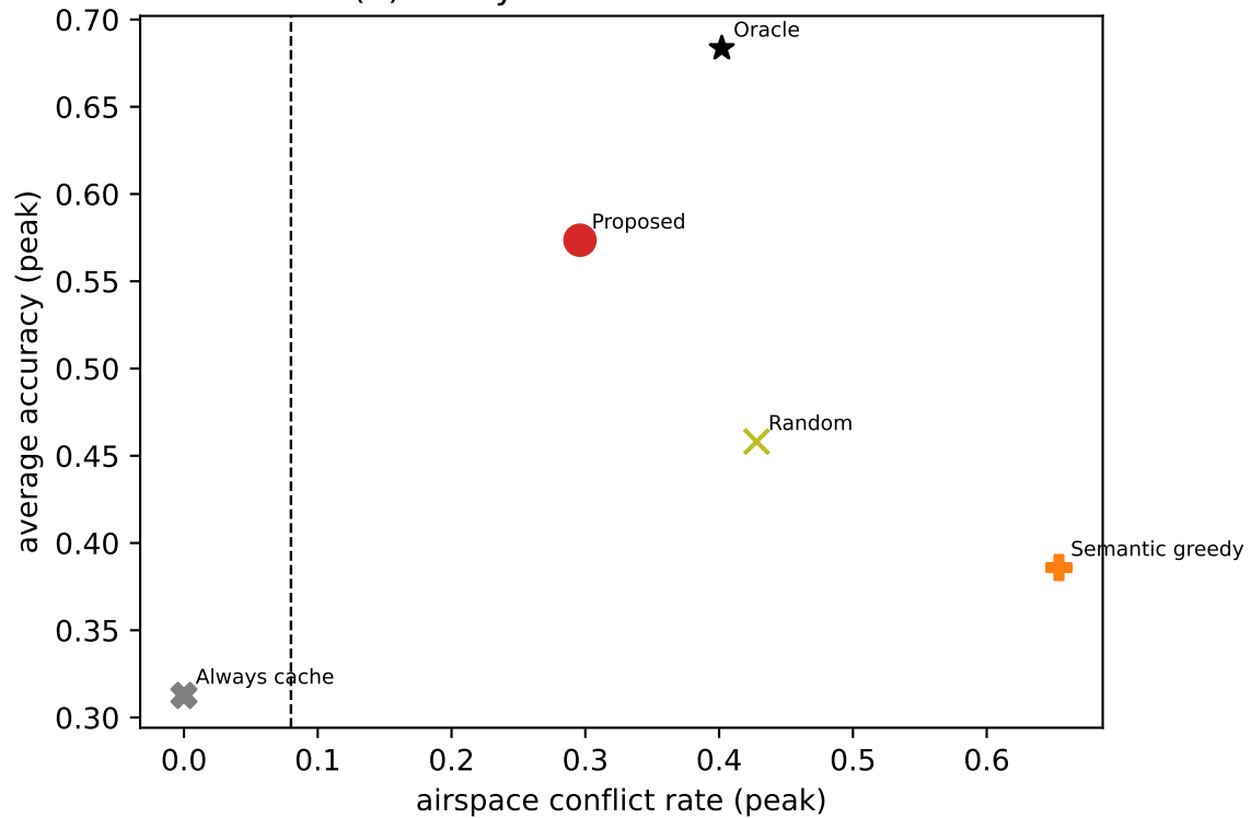
(b) Utility-violation Pareto view
