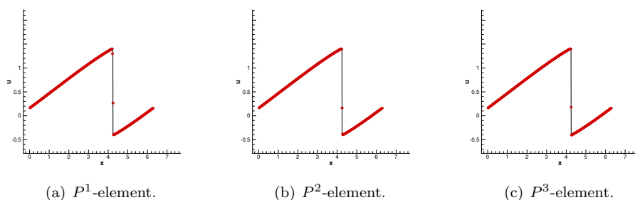
FIG. 4.2. The numerical solution with final time T = 2.2 in Example 2.
