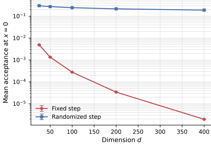
Figure 1: Estimated mean acceptance probability at the origin for the target (17). Fixed-step MALA uses h = h_0 , while randomized-step MALA uses h \sim \text{Unif}(0, h_0) . The vertical axis is logarithmic, and vertical bars show \pm 2 estimated standard errors; most are narrower than the markers.
